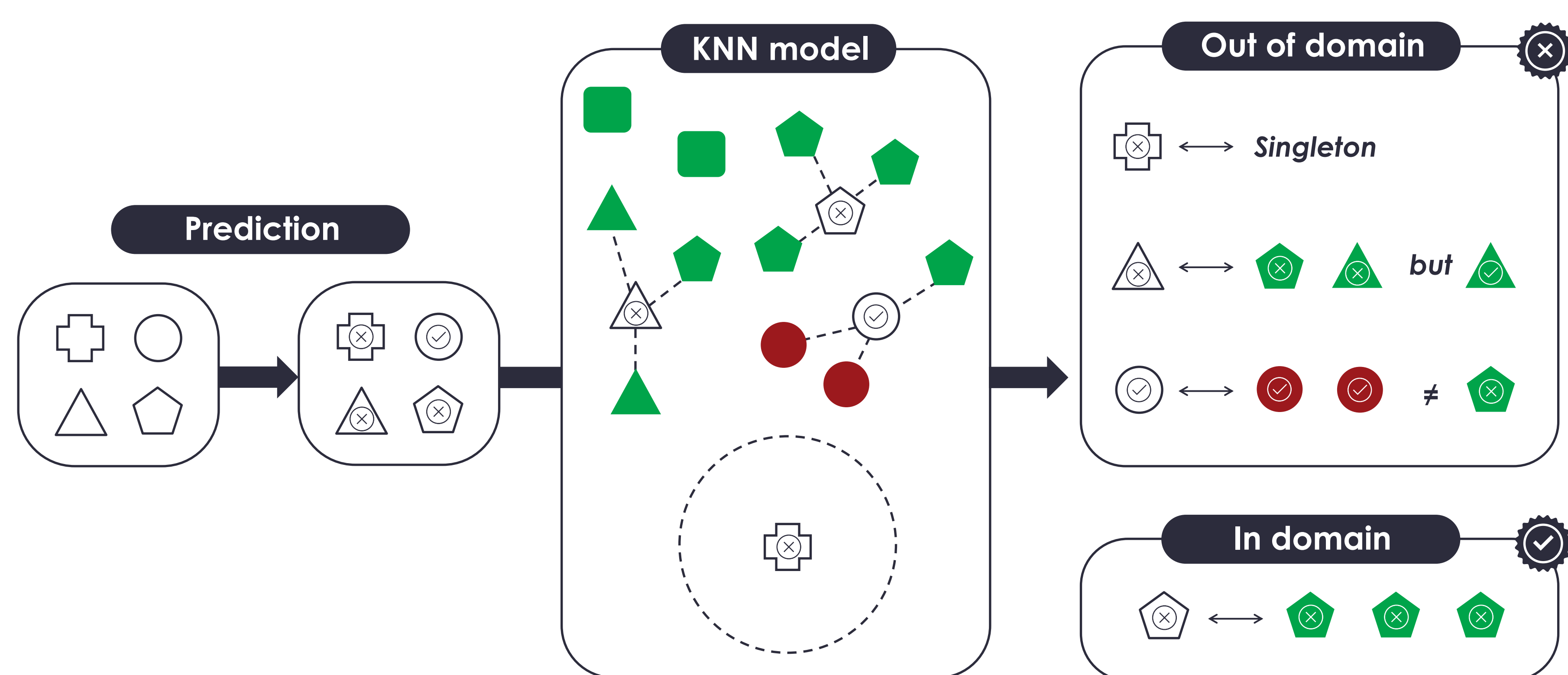
Figure 2. Applicability domain is defined by a k-nearest neighbours' model (KNN). The predicted substance (white shape) is defined as out of domain whenever no analogues (coloured shapes) are retrieved. To be in domain, at least one analogue must be retrieved. Furthermore, prediction for each analogues (in white, within the coloured shape) must be similar to their respective experimental value (green for inactive, red for active) and match the prediction for the query substance.
